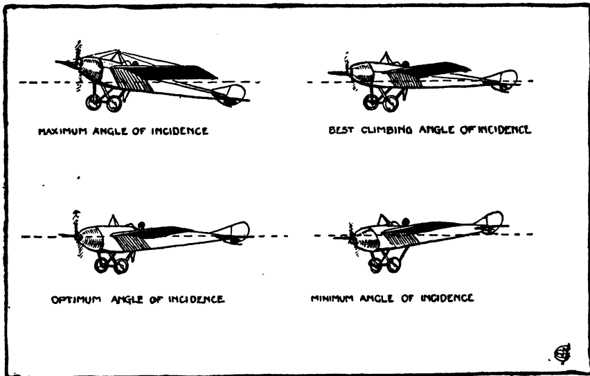
The angles shown above are only roughly approximate, as they vary with different types of aeroplanes
